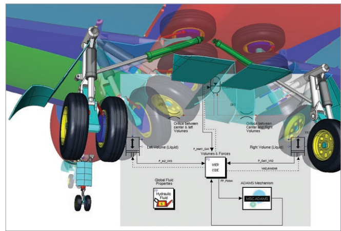
Go beyond fit to function with Easy5
