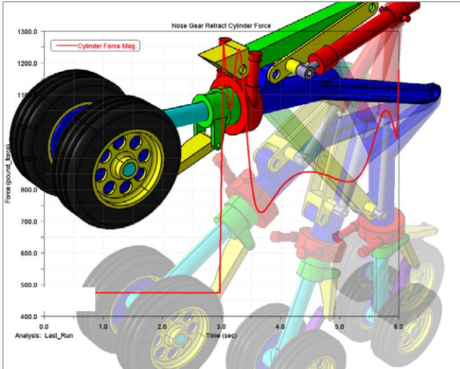
Adams Easy5 co-simulation
